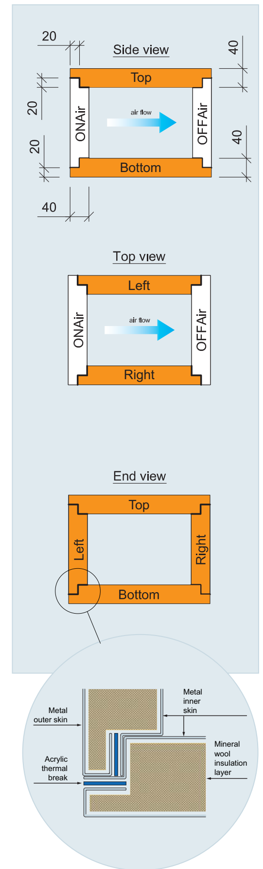
Frameless casing connection
