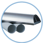
MICRA 200 chrome mounting kit: • two plastic \varnothing 100 mm air ducts 500 mm long • outdoor box (white) • cardboard template
